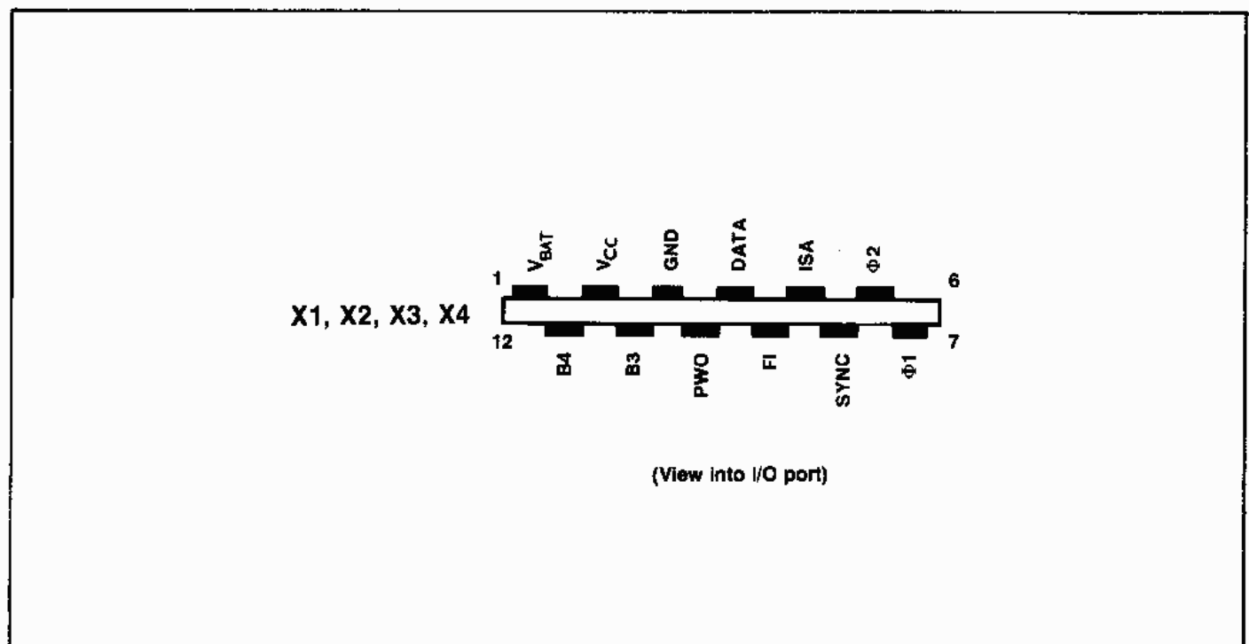
Figure 4-6. Contacts at I/O Port
