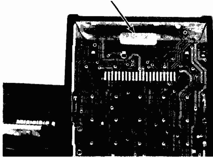
Figure 7-1. Halfnut Display Hybrid IC
