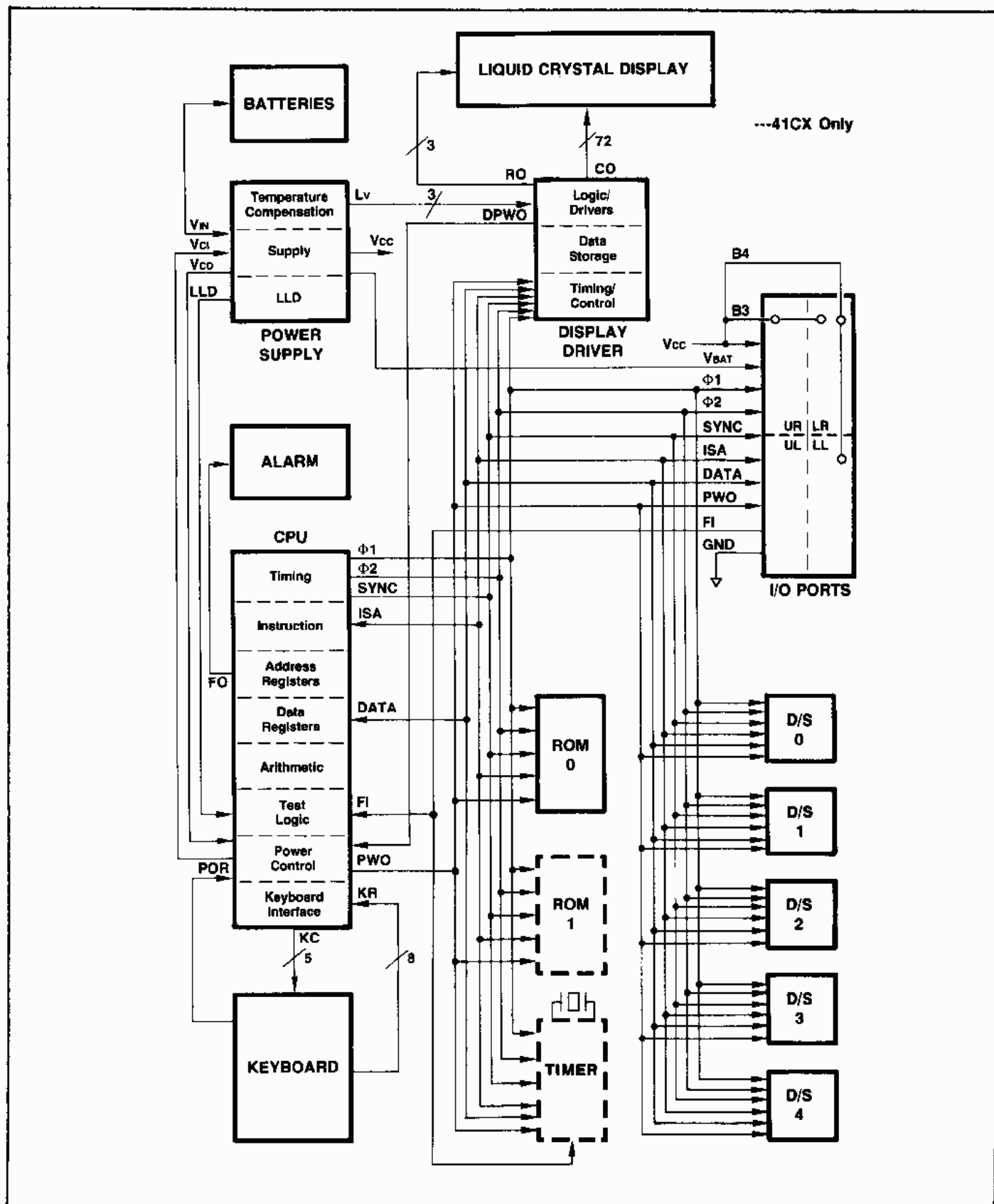
Figure 2-2. HP-41C/CV/CX Common Board Block Diagram
