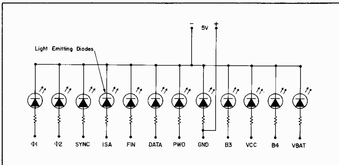
Figure 4-4. Port Extender Modification Schematic
