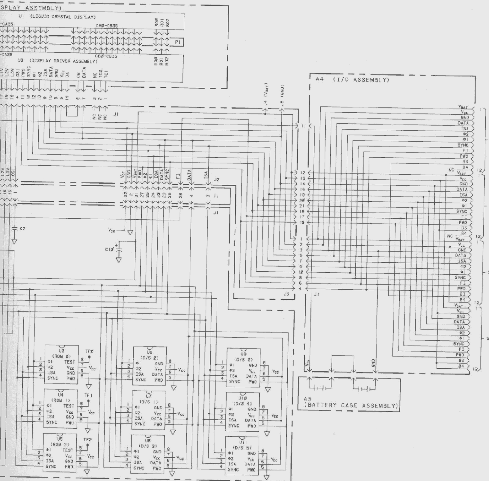
Figure 4-9d. Initial HP-41CV Schematic Diagram
