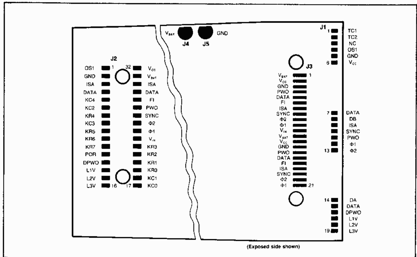
Figure 4-5. Contacts on Keyboard PC Board
