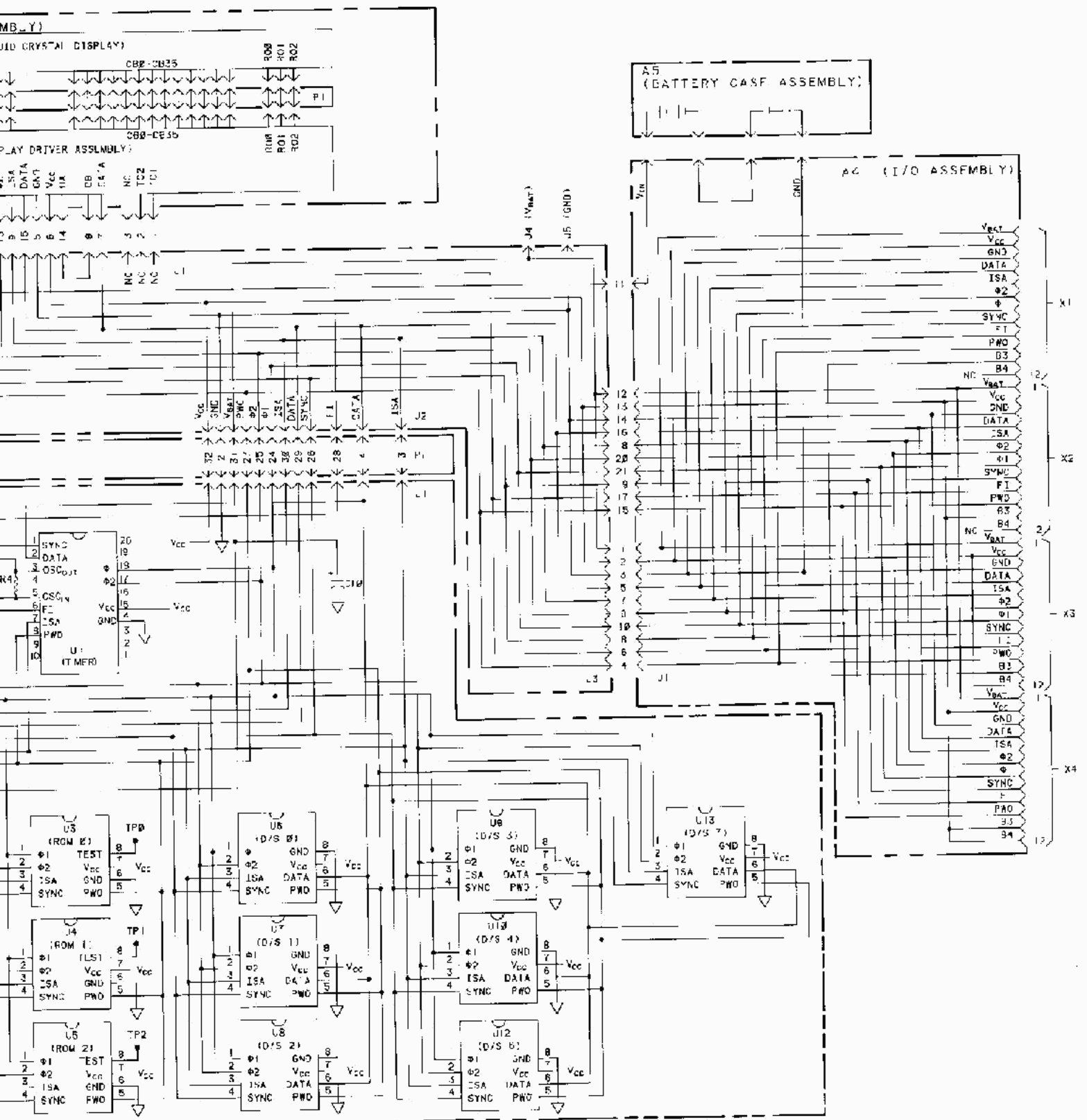
Figure 4-9f. HP-41C/CV/CX Common Board Schematic Diagram
