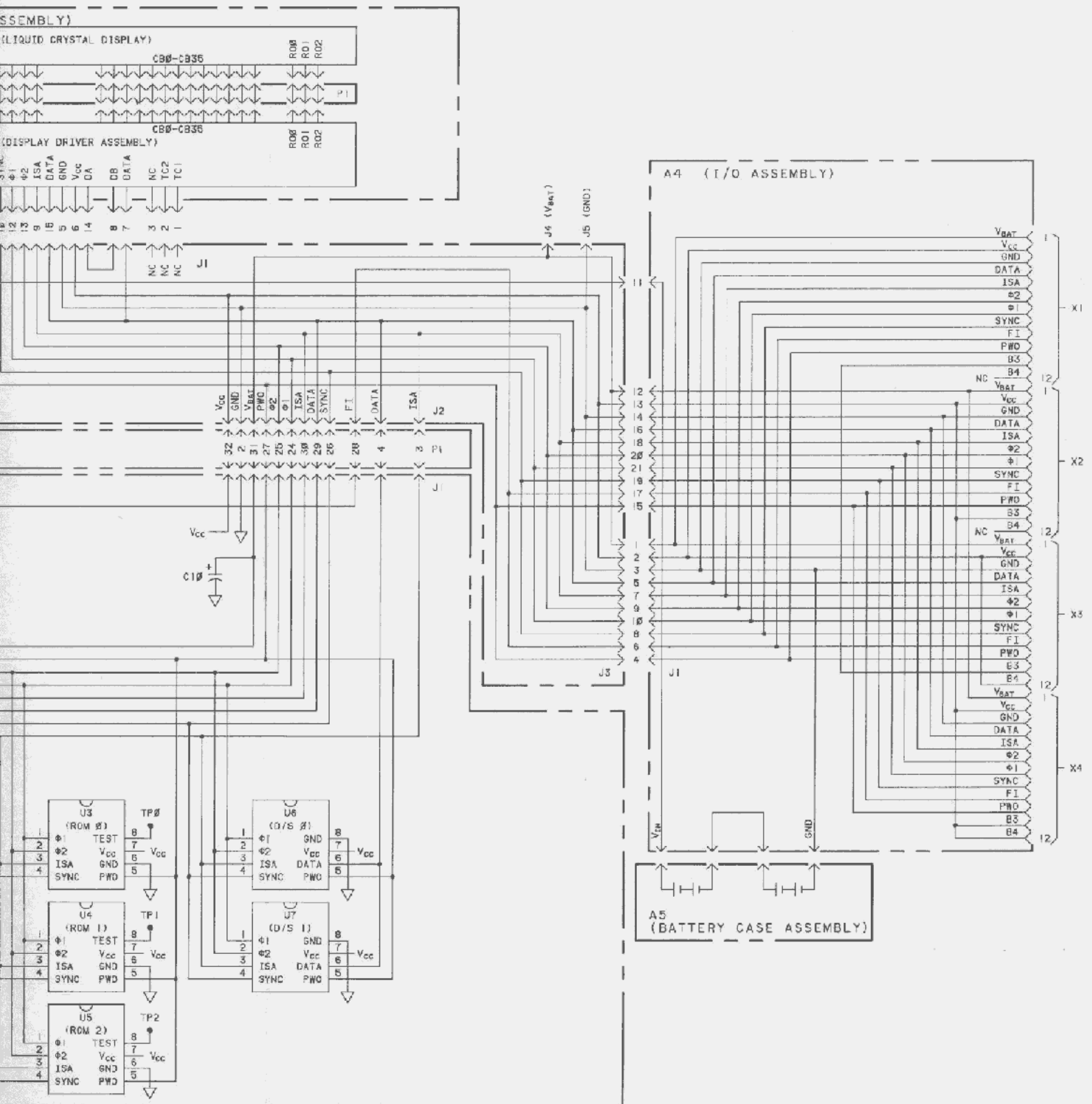
Figure 4-9c. Final HP-41C PCA Schematic Diagram
