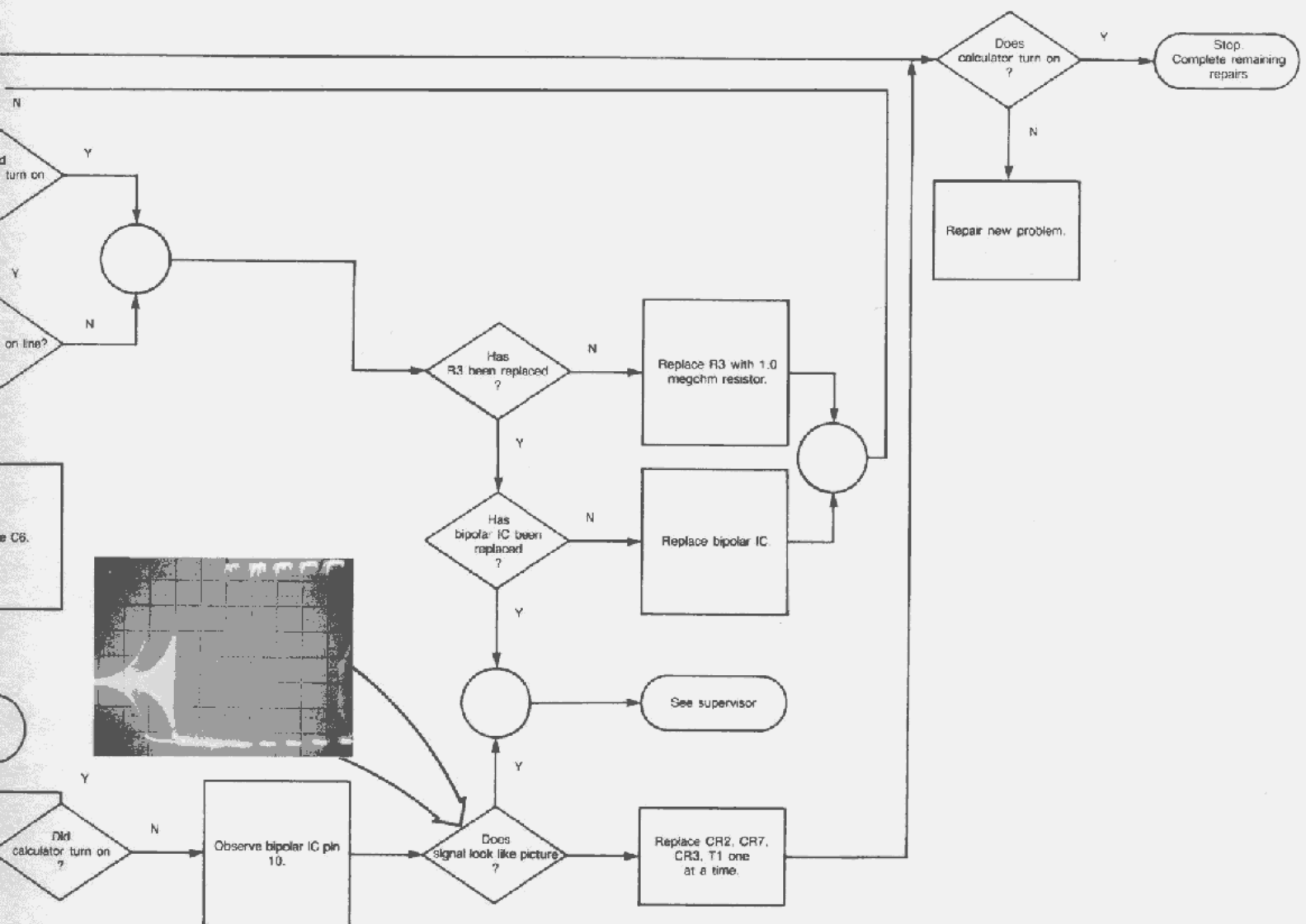
Figure 4-3. Power Supply Troubleshooting Flow Chart
