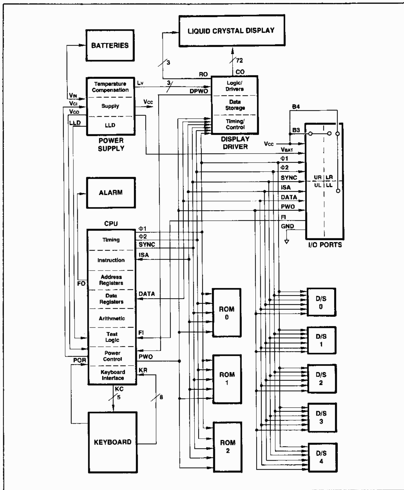
Figure 2-1. HP-41C/CV Block Diagram
