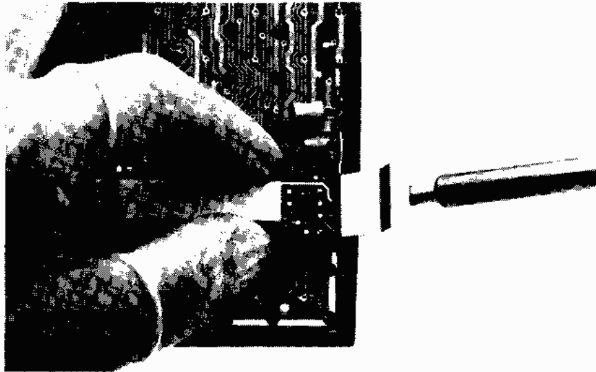
Figure 7-7. Blade-Shaped Soldering Iron Tip in Use
