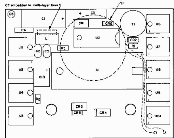
Initial HP-41CV
