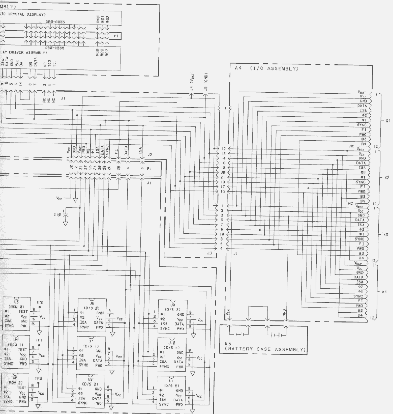
Figure 4-9e. HP-41C/CV Common Board Schematic Diagram
