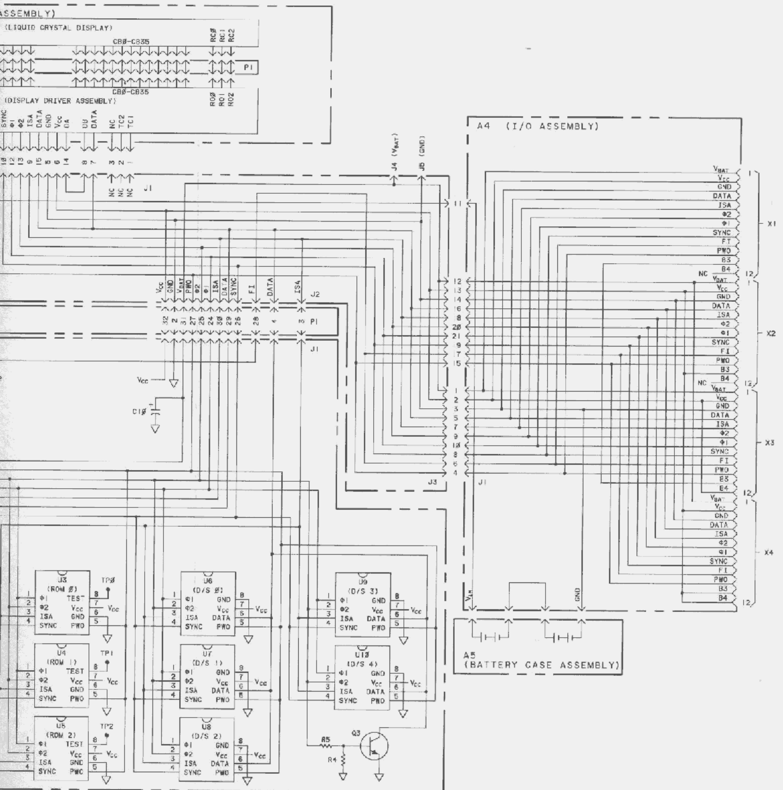
Figure 4-9a. Initial HP-41C Schematic Diagram
