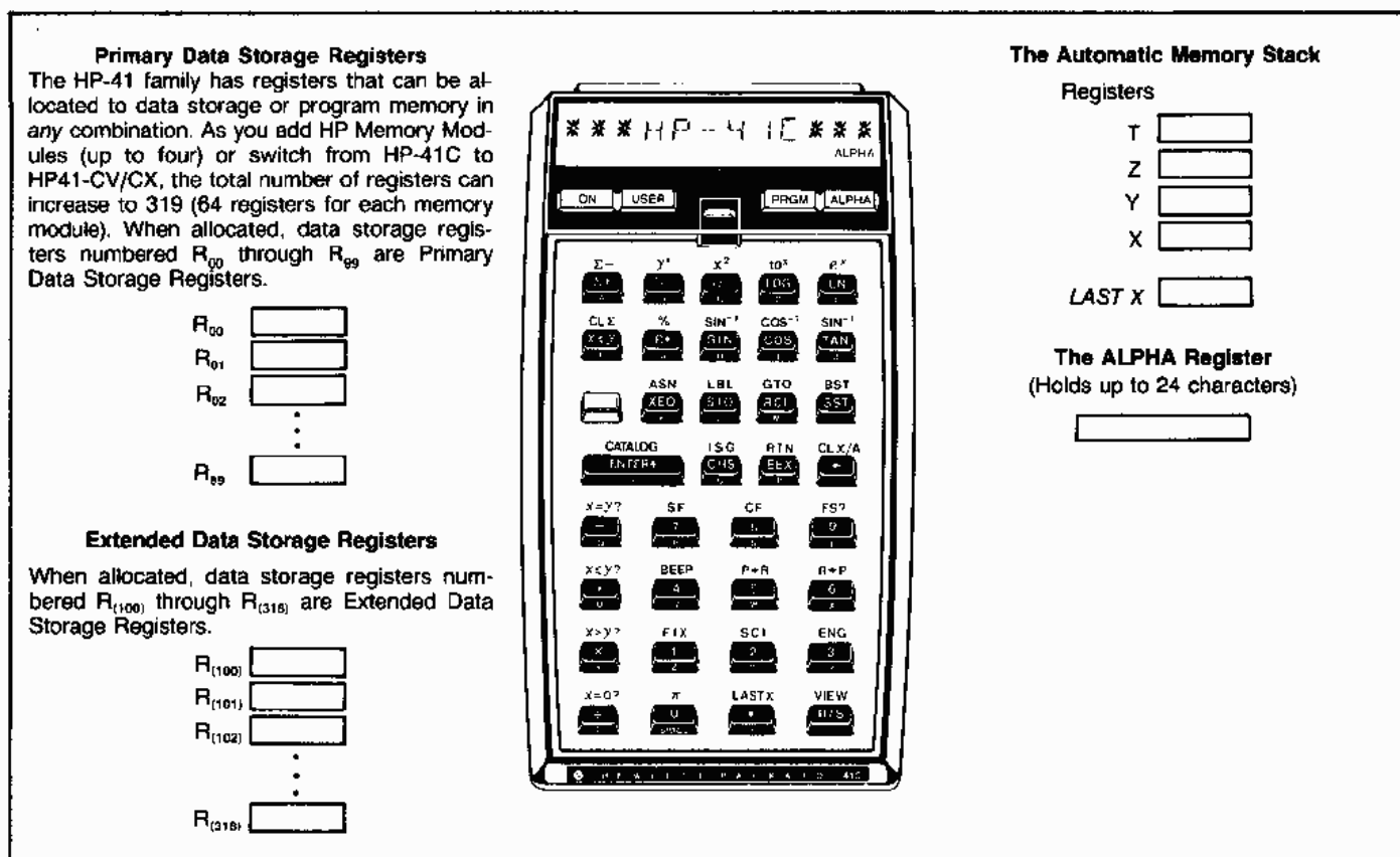
Figure 1-1. HP-41 Keyboard
