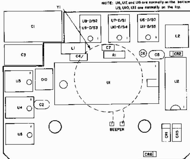
HP-41C/CV Common Board
