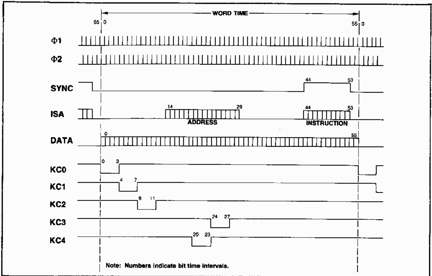
Figure 2-4. System Timing
