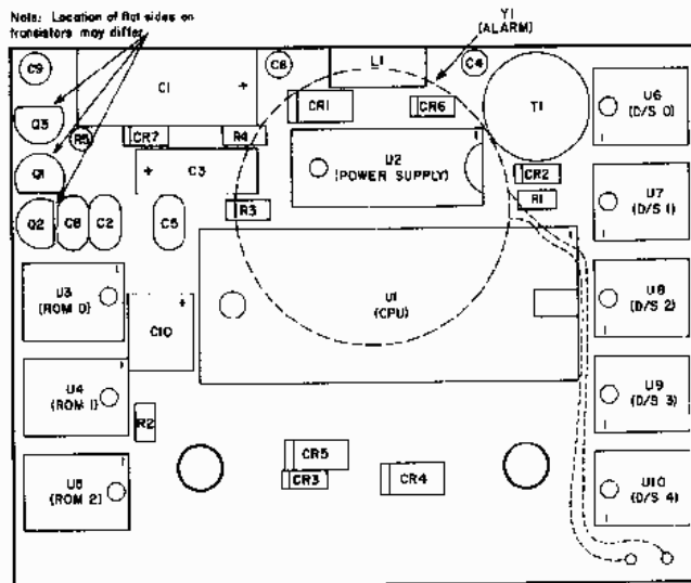
Initial HP-41C
