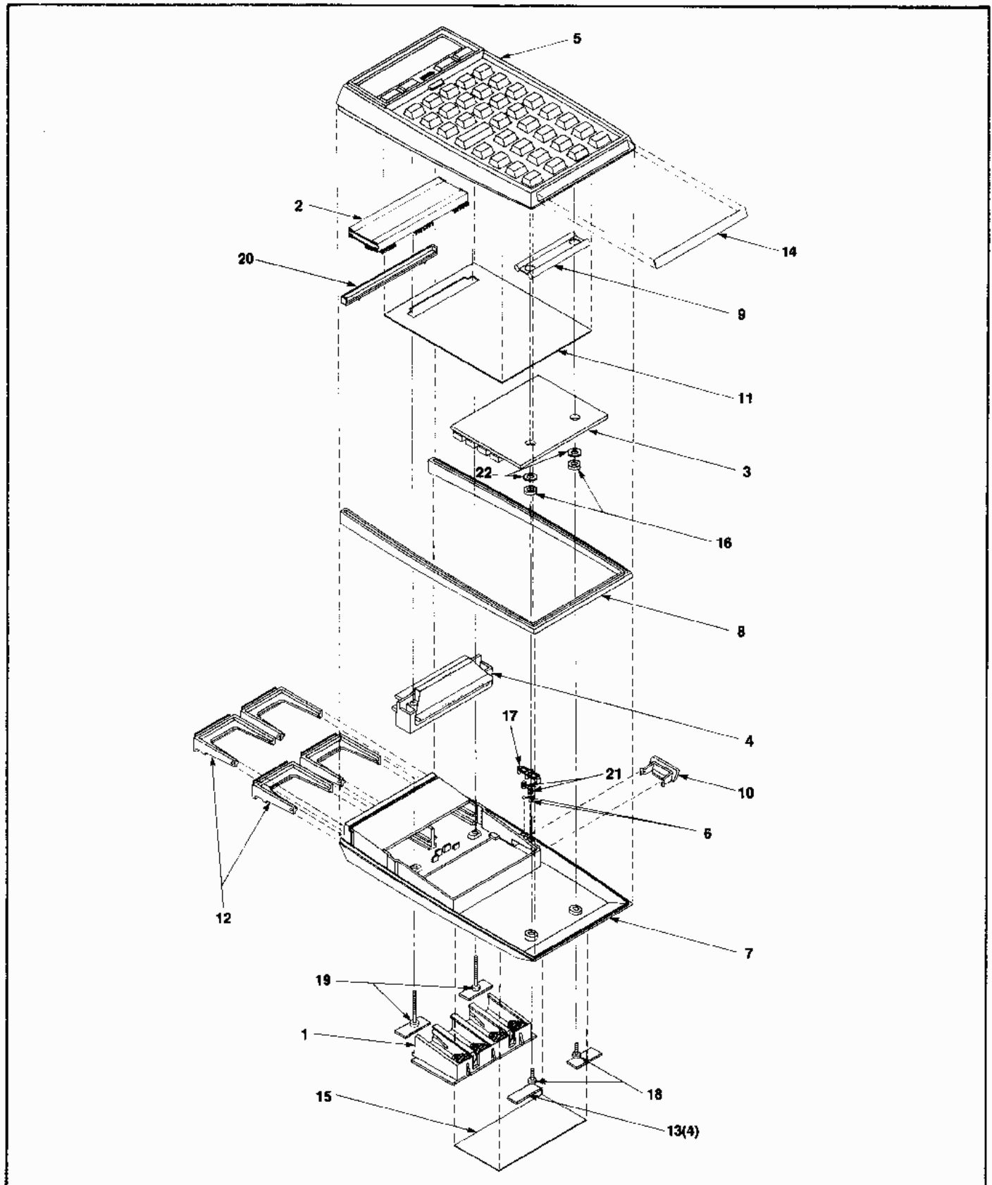
Figure 6-1. HP-41 Exploded View
